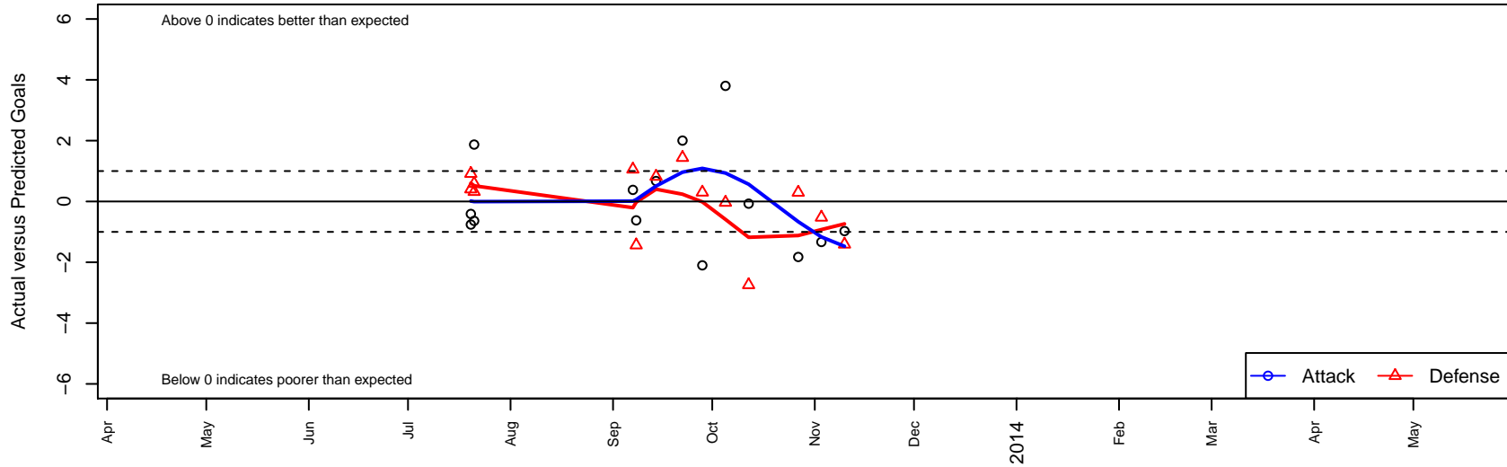
Riverside FC Blue B95 Dots are actual minus expected GF (blue circles) and GA (red triangles). Blue line is smoothed change in attack strength. Red is smoothed change in defense strength.
